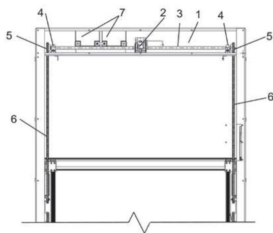
Fig. 6. Drive of the closing/opening mechanism: 1 – top case profile; 2 – gear motor with a direct current electric drive; 3 – drive shaft; 4 – bearing support; 5 – chain sprockets; 6 – cable chains; 7 – emergency power supply batteries
