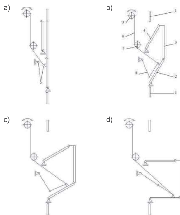
Fig. 2. Kinematic diagram of the window-to-balcony module: a – closed position (window); b – tilted position 1 (30°); c – tilted position 2 (60°); d – open position (balcony); 1 – external wall of a building; 2 – balcony decking; 3 – balustrade; 4 – balustrade handrail; 5 – flexible cable drive system; 6 – flexible cable; 7 – passive roller; 8 – articulated rigid rod
