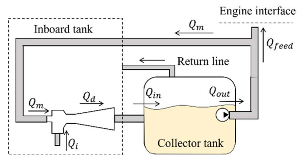
Fig. 6. Jet pump and collector tank flow balance
