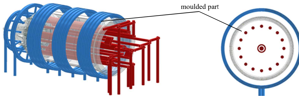
Fig. 3. 3D model of mould cooling: blue – cooling of the die; red – cooling of the punch
