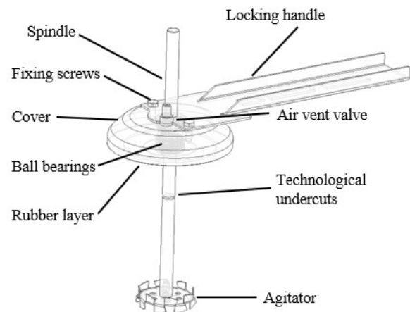
Fig. 2. Construction of a mixing and deaeration device for adhesive compositions
