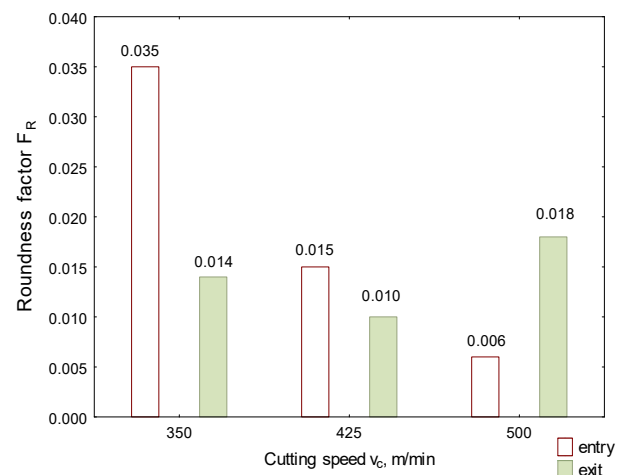
Fig. 6. Roundness factor F_R for the Al/CFRP strategy after milling
