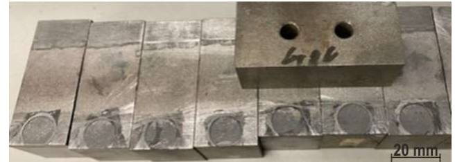
Fig. 12. Cohesive destruction of Raex 400 material samples with a diameter of 12.6 mm
